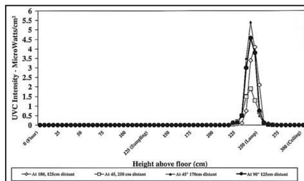
FIGURE 3. Intensity of the upper air ultraviolet germicidal irradiation (UVC) from a wall-mounted fixture by height from the floor, as well as the angle and distance from the fixture.
